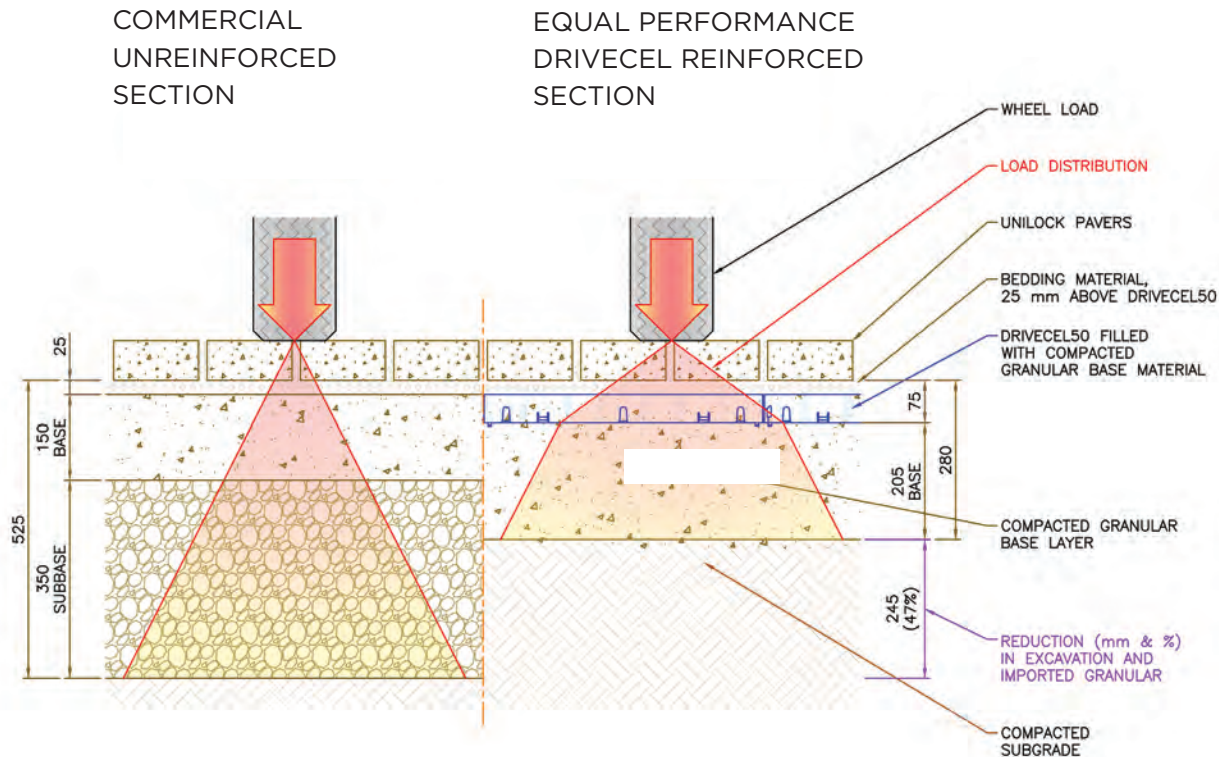
DRIVECEL GF50 HEAVY DUTY - LOAD DISTRIBUTION
