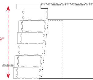
Walls (24" - 39")
