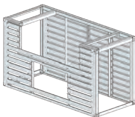
Grill Module - Front and Back Model: UNI.05.A000 NAV: RS-UCARA001003 64 1/2 x 27 1/2 x 36"
